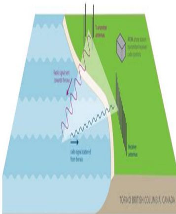
ONC'S HIGH FREQUENCY OCEANOGRAPHIC WERA RADAR
